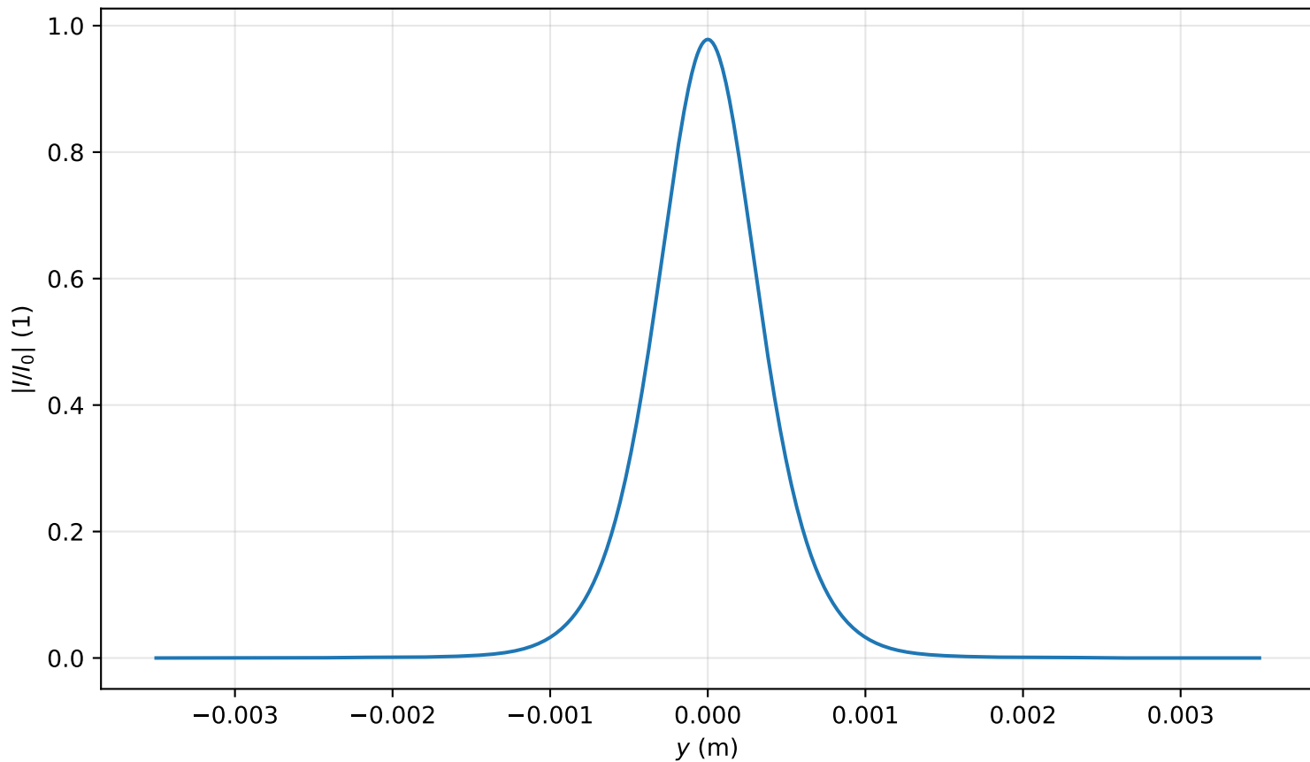
Intensity profile I(x=0, y, z=3.503)/I_0 , \text{Pin}=0.8\text{Pcr} , artificial time
